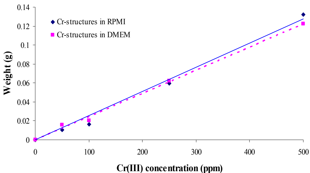
Figure 5.6: Effect of the concentration of Cr(III) on the weight of Cr(III) complexes. RPMI 1640 ( R^2=0.989 ) and DMEM high glucose ( R^2=0.997 ) media were incubated with Cr(III) from 0 to 500 ppm. Pellets obtained after centrifugation were air dried and weighted.
