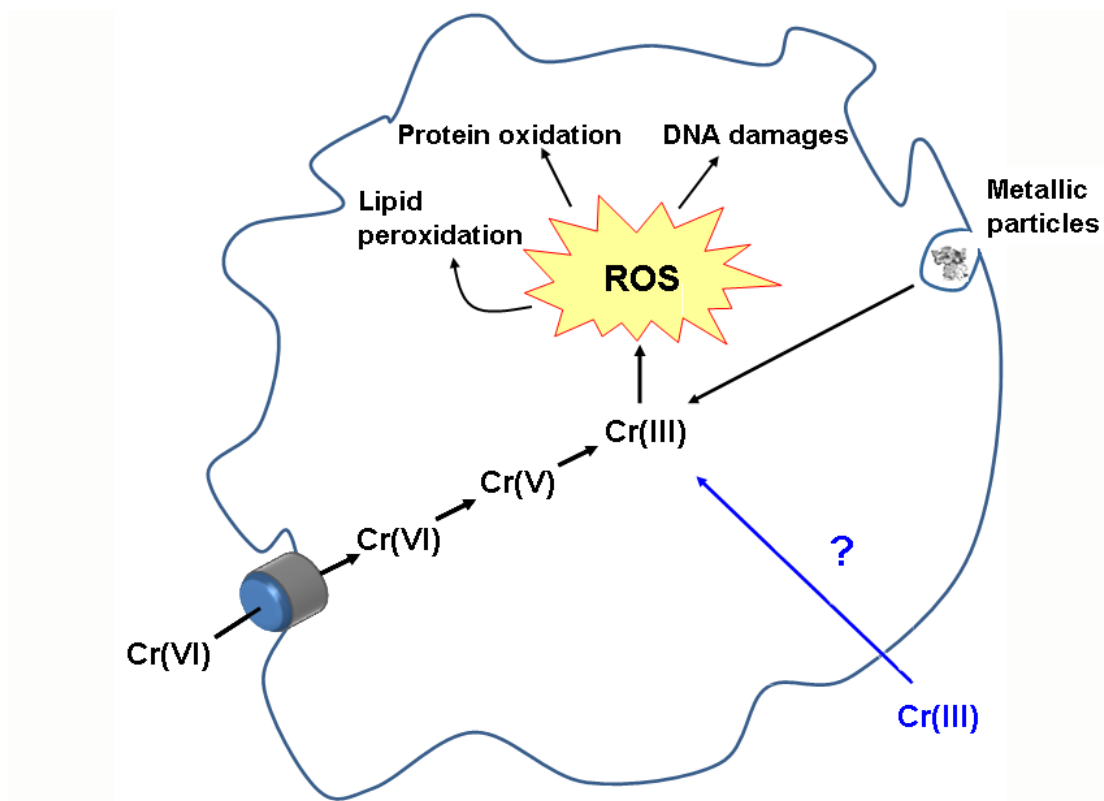
Figure 3.4: Hypothetic scheme used to illustrate the Cr ions internalization pathways.
