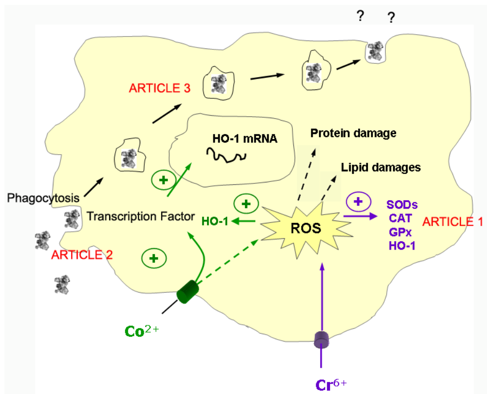
Figure 8.4: Effects of Cr(III), Co(II), and Cr(VI) in cells: A model.
