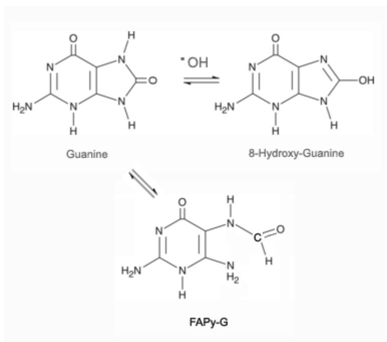
Figure 3.9: Modification of Guanine by ROS.
