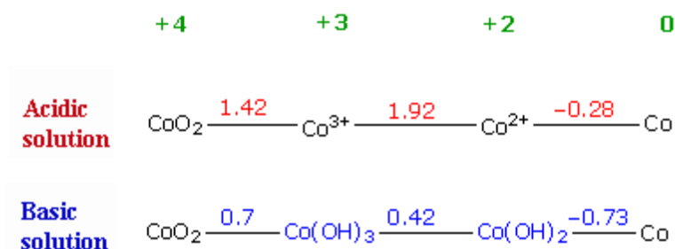
Figure 3.3. Standard reduction potentials for cobalt.
