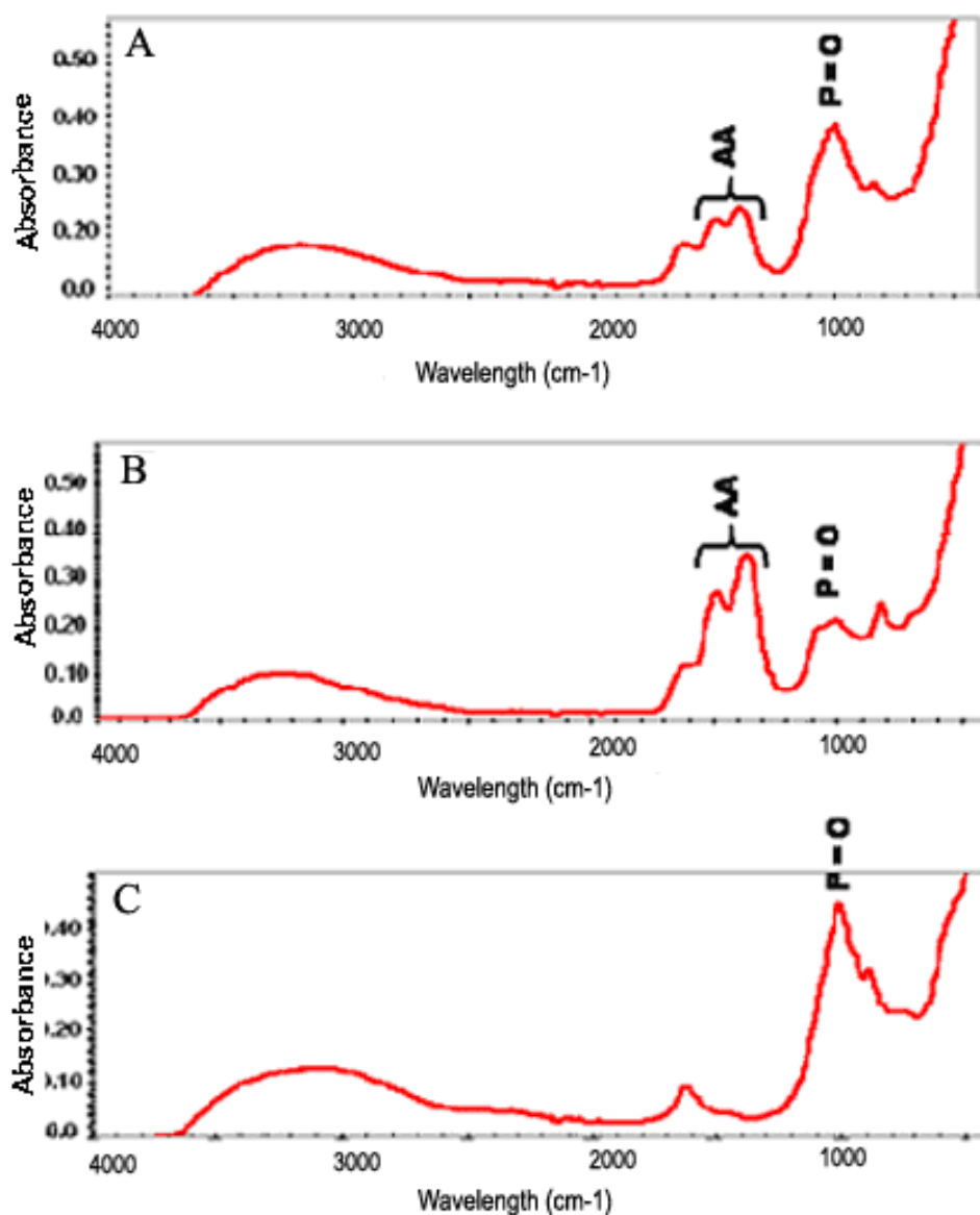
Figure 5.5: Analysis of Cr(III)-complexes by ATR FT-IR. Cr(III) complexes obtained in RPMI 1640 (A) and DMEM high glucose (B) were compared to CrPO 4 (C). AA: amino acid characteristic pics.
