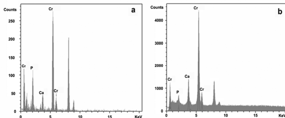
Figure 6.4: EDXA spectra of Cr(III) complexes internalized by U937 macrophage-like cells in RPMI 1640 with FBS (a) and in DMEM high glucose supplemented with FBS (b). EDXA spectra obtained in HS are the same (data not shown). Copper peaks visible on the right of the spectra (8-9 keV) are generated by the grids. Note the presence of chromium (Cr), phosphate (P) and calcium (Ca) in both Cr(III) complexes.
