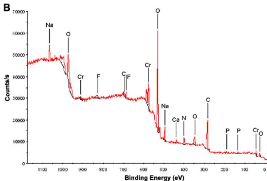
Figure 5.7: X-ray photoelectron spectroscopy analysis of Cr(III) complexes.
