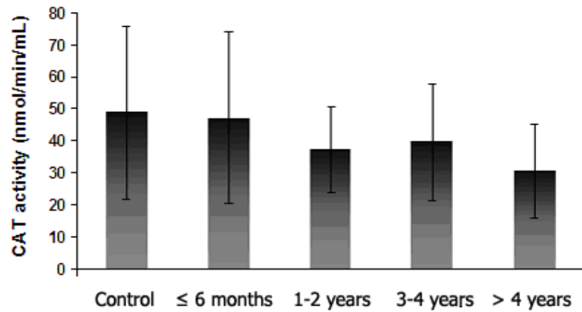
Figure 7.6: Catalase (CAT) activity in the plasma of patients with MM THAs. CAT activity was measured in the plasma of patients with 28 mm-head MM prosthesis up to 10 years post-operatively. Results are expressed as the mean \pm standard deviation.
