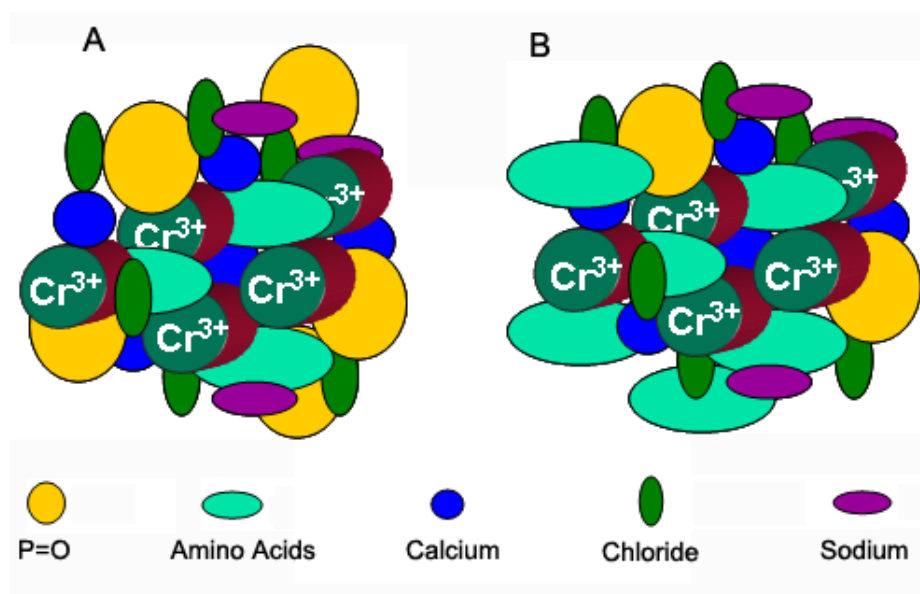
Figure 8.1: A proposed model for the nanoscale Cr(III) complexes formed in RPMI 1640 (A) and DMEM high glucose (B) media. The main difference between the complex A and the complex B is the ratio between amino acids and phosphates. Complexes A contain more P=O and less amino acids than complexes B.
