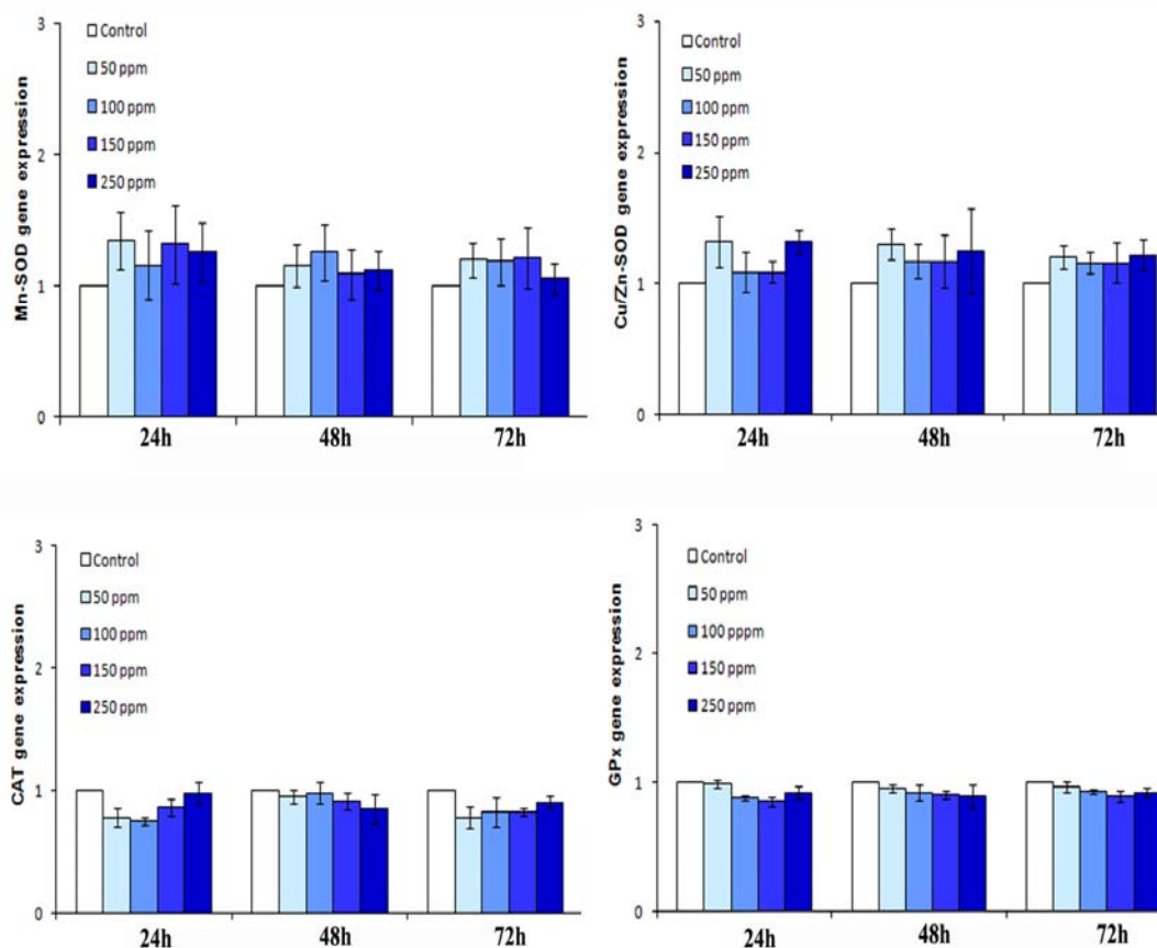
Figure 4.5: Effect of Cr(III) on the gene expression of antioxidant enzyme.
