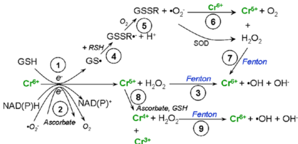
Figure 3.5: Biological reduction of \text{Cr}^{6+} and the different associated reactions producing ROS.
