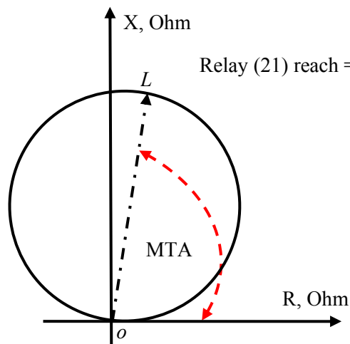
Figure 2.11. A mho distance relay characteristic.
