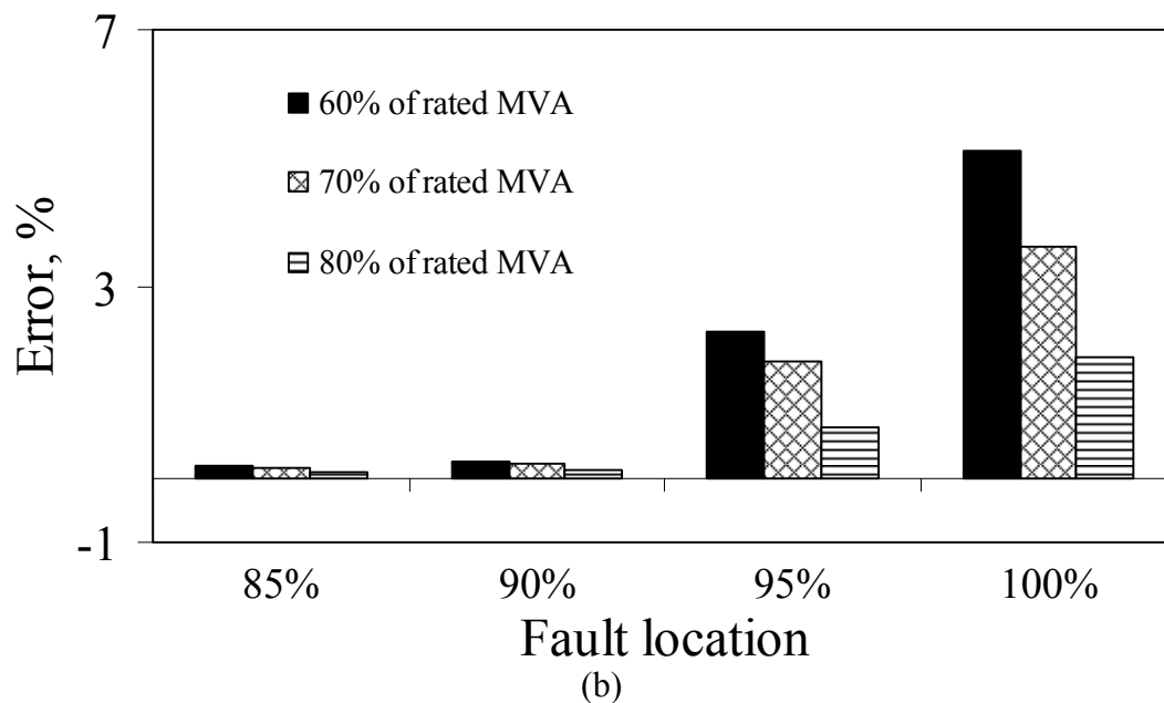
Figure 2.27. PEMI for three-phase faults on Line 1 in System II: (a) with a midpoint STATCOM, (b) with a midpoint SVC.
