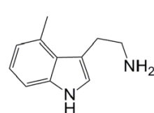
5-methyltryptamine
