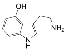
5-Hydroxytryptamine
