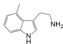
5-methyltryptamine
