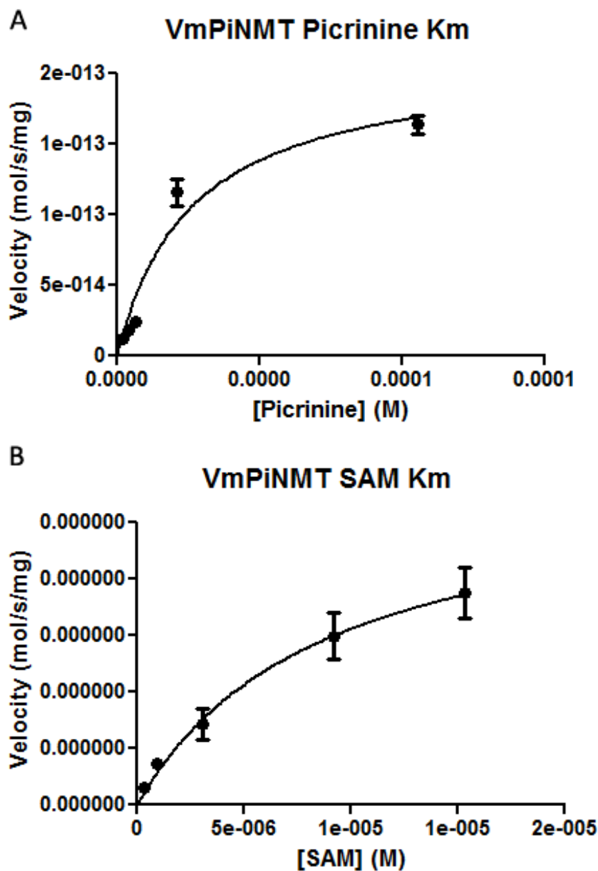
Figure A-11. Michaelis–Menten plots of kinetic data for VmPiNMT. Nonlinear regression analysis of kinetic data were used to estimate kinetic parameters for VmPiNMT with substrates (A) picrinine, and (B) S-adenosyl-L-methionine (SAM).
