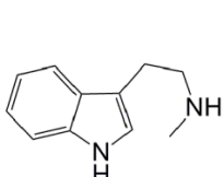
N-methyltryptamine
