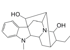
Ajmaline
