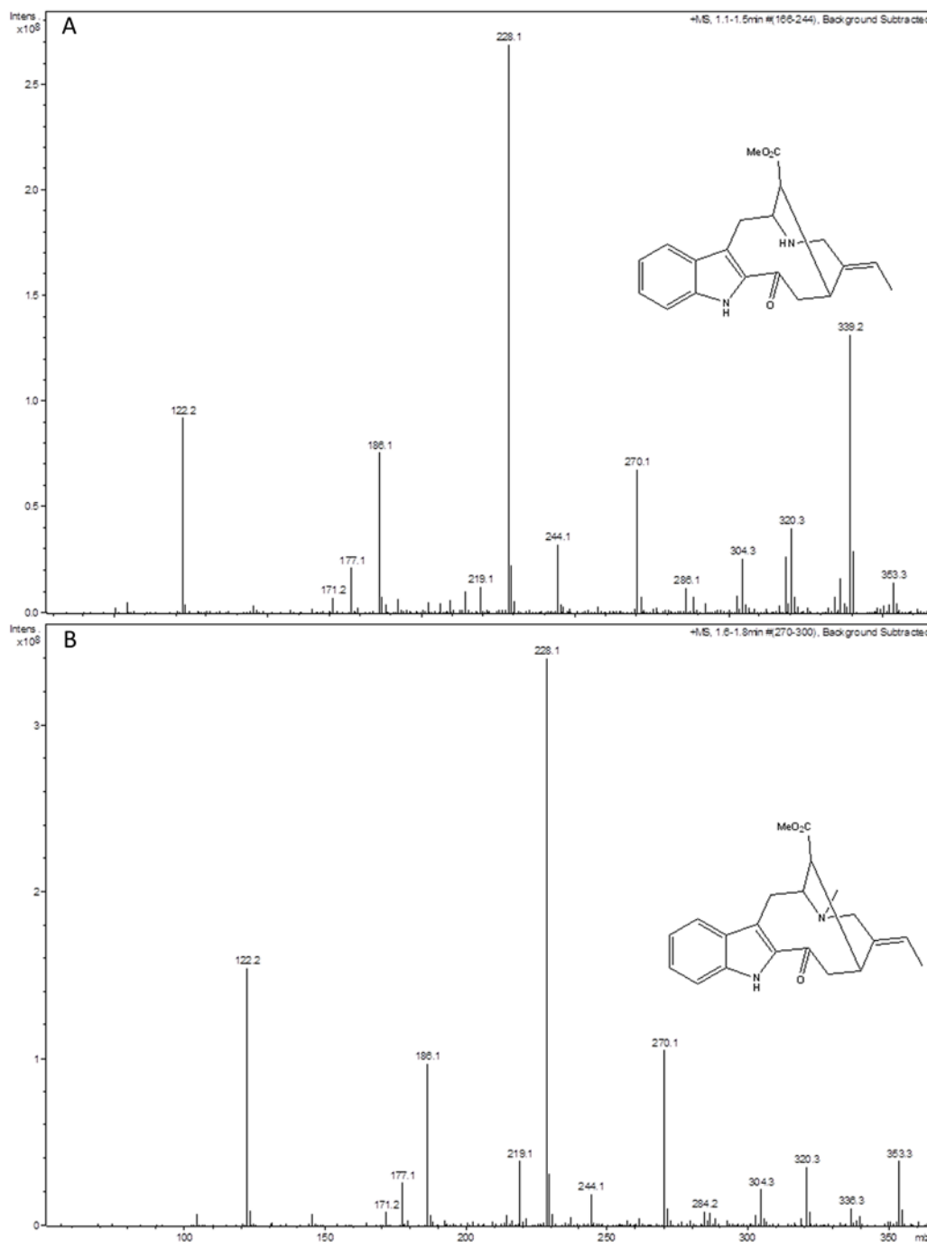
Figure A-1. MS1 analysis of alkaloid products of cell free pET 30b-EV (A) and recombinant CrPeNMT (B) methyltransferase assay products supplied with perivine standard as substrate.
