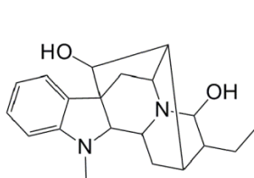
Ajmaline
