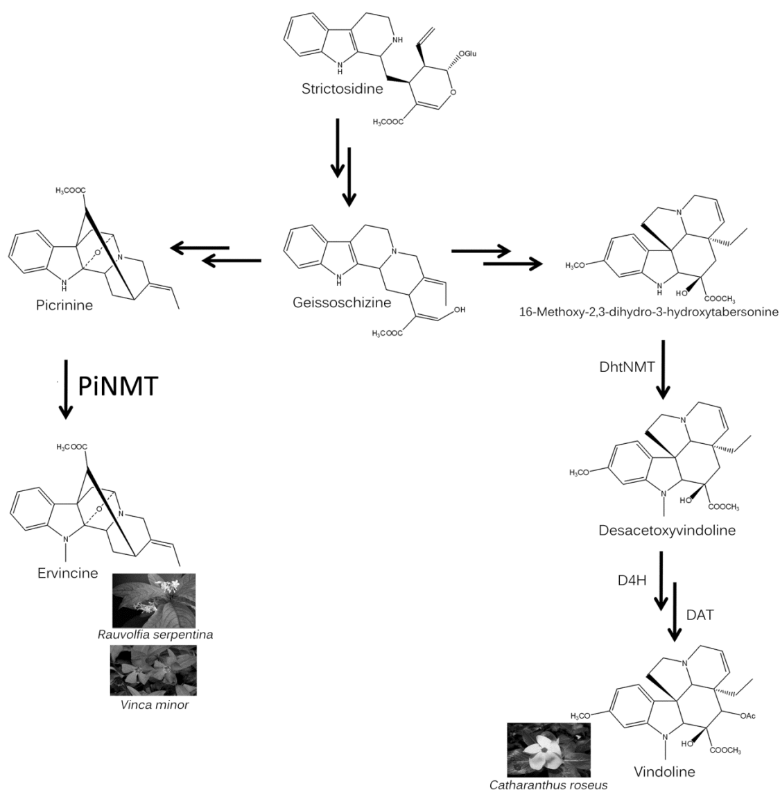
Figure 5-1. Possible biochemical pathway for conversion of Strictosidine to Various N -Methylated MIAs in Apocynaceae
