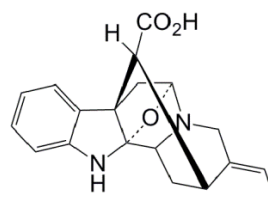
Picrinine
