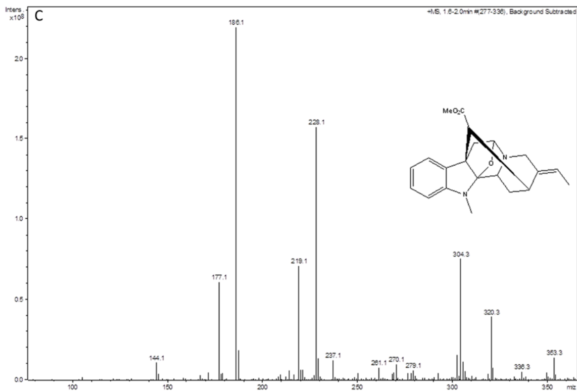
Figure A-5. MS1 analysis of alkaloid products of cell free pET 30b-EV (A), recombinant VmPiNMT (B) and recombinant RsPiNMT (C) methyltransferase assay products supplied with picrinine standard as substrate.
