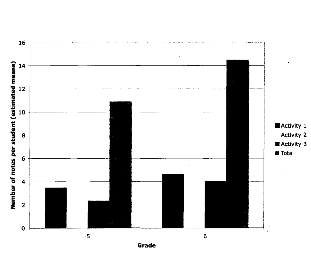
Figure 7. Multivariate effect of grade (Site A, n = 29 ).
