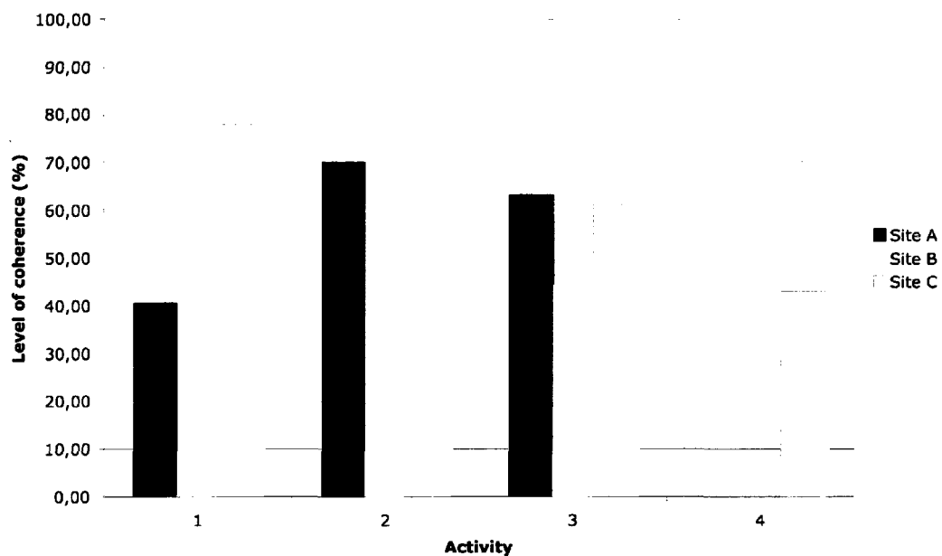
Figure 17. Level of coherence in scaffold use across sites and activities.
