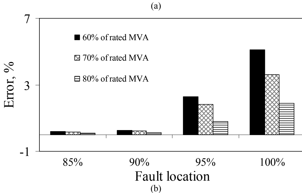
Figure 2.27. PEMI for three-phase faults on Line 1 in System II: (a) with a midpoint STATCOM, (b) with a midpoint SVC.
