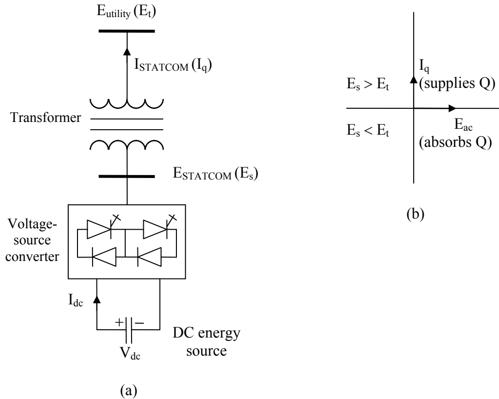
Figure 2.6. The STATCOM principle diagram: (a) power circuit, (b) reactive power exchange.
