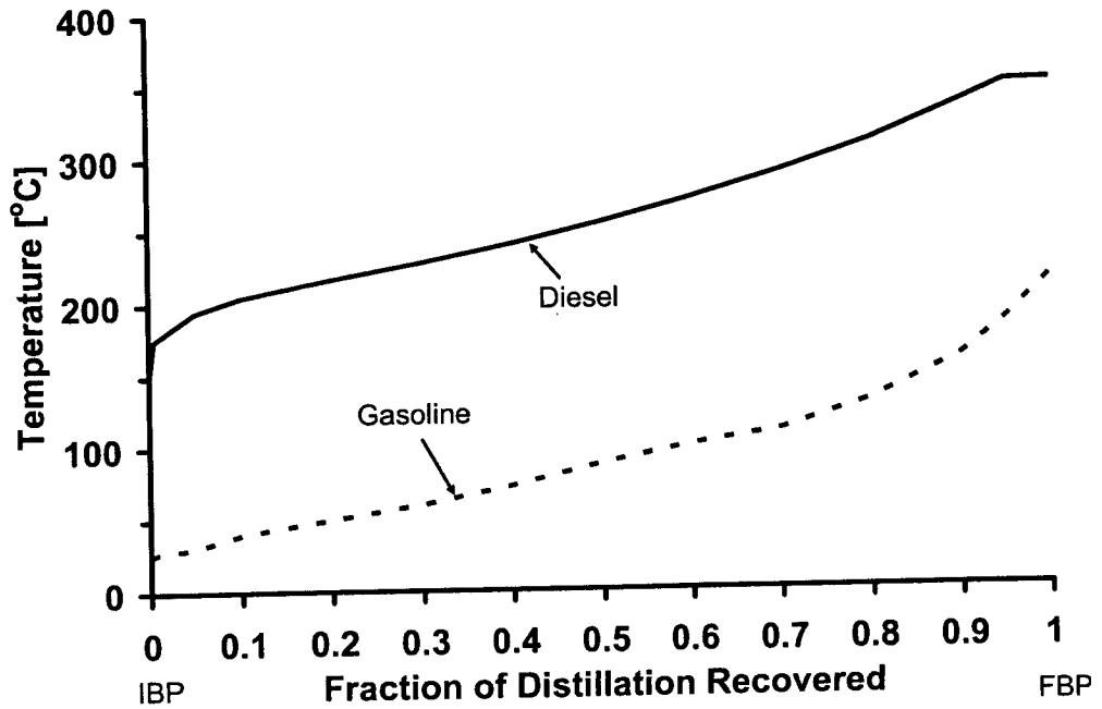
Figure C-3: Distillation Curve of Diesel and Gasoline
