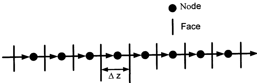
Figure 3-8: Staggered Mesh Formation
