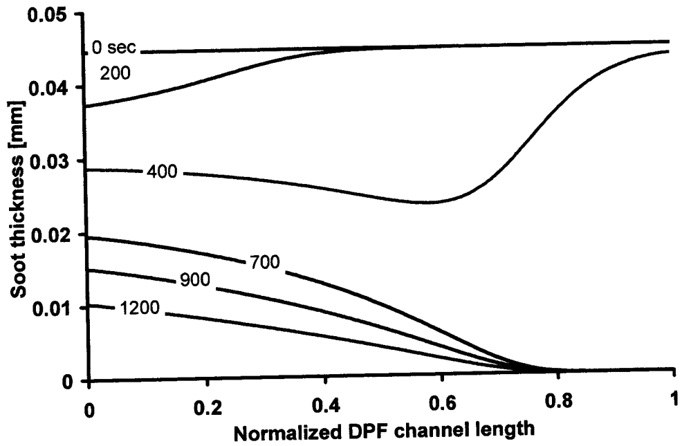
Figure 4-21: Soot Oxidation Simulation (Case S2B)
