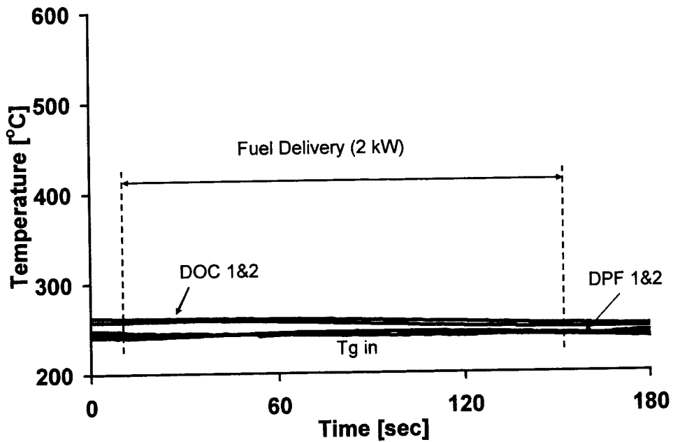
Figure 4-6: Experimental Result (Case T1)
