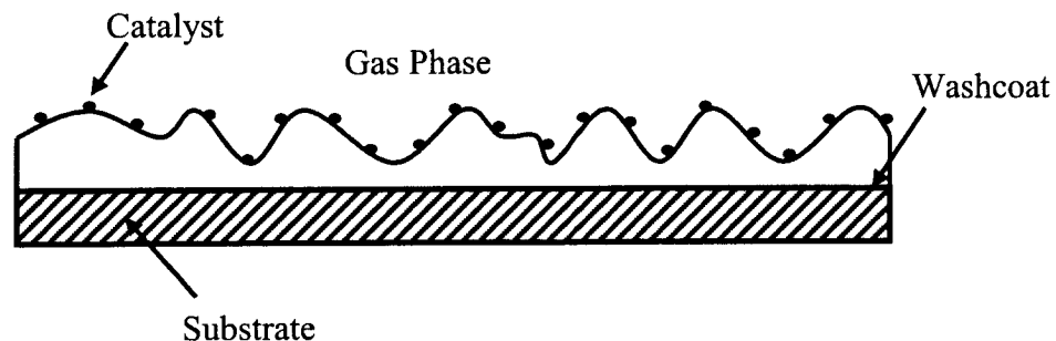
Figure 2-4: Representation of Catalyst Dispersed in Washcoat of DOC Channel
