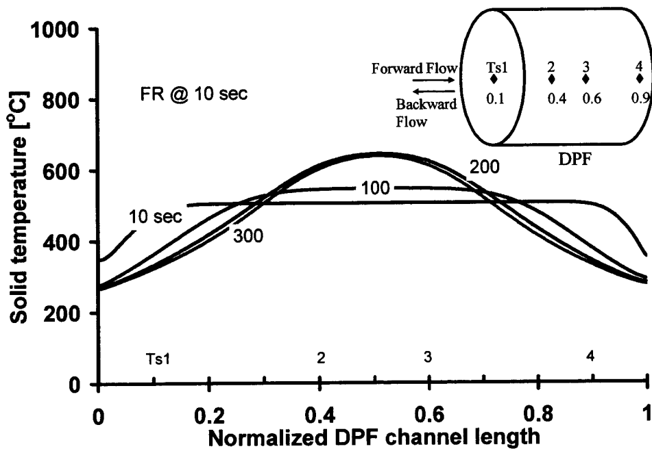
Figure 4-16: Temperature Profile (FR)
