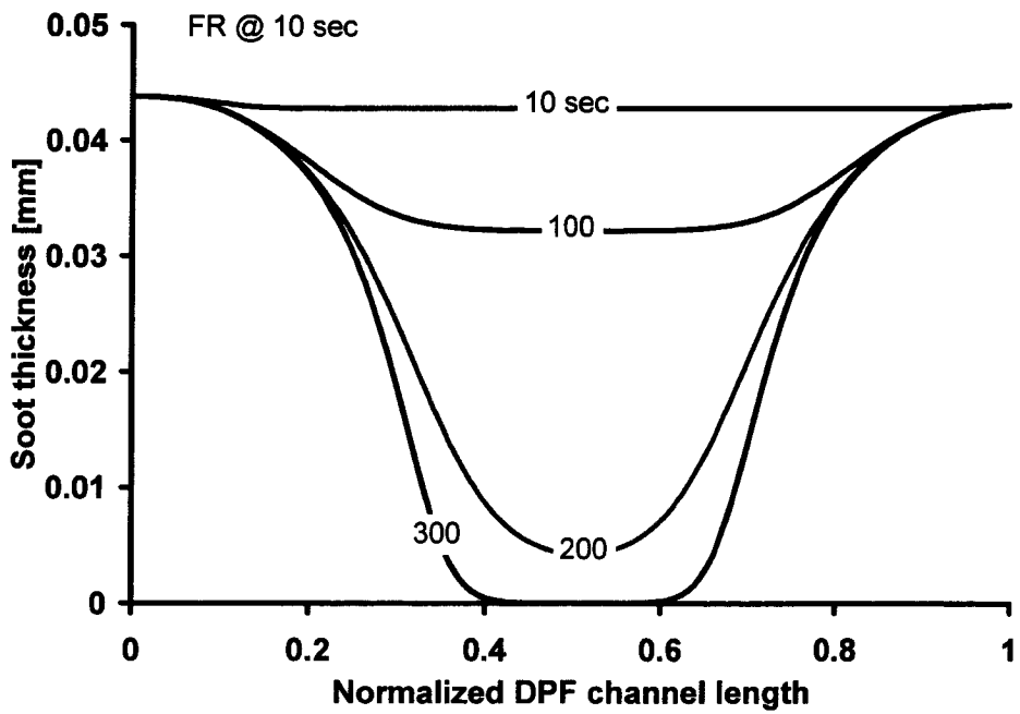
Figure 4-14: Soot Profile (FR)
