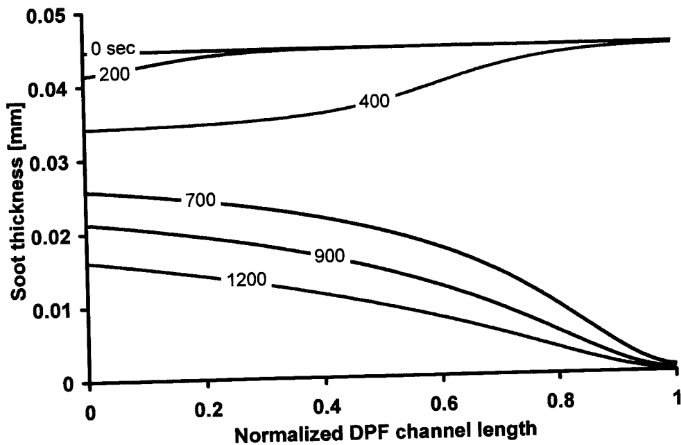
Figure 4-23: Soot Oxidation Simulation (Case S2C)
