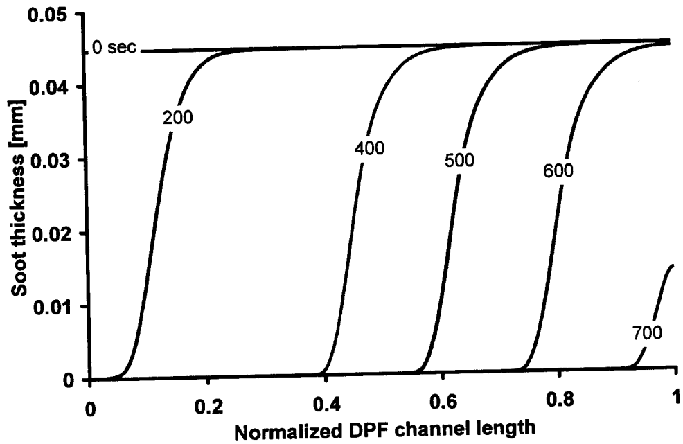
Figure 4-27: Soot Oxidation Simulation (Case S3B)
