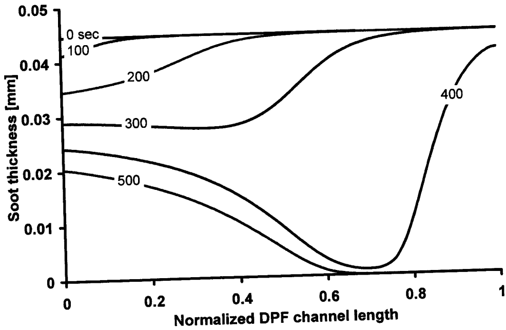
Figure 4-19: Soot Oxidation Simulation (Case S2A)
