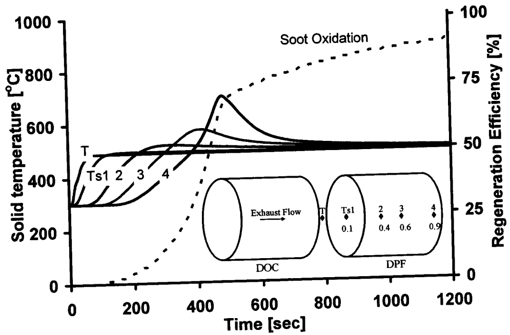
Figure 4-20: Transient Simulation Results (Case S2B)
