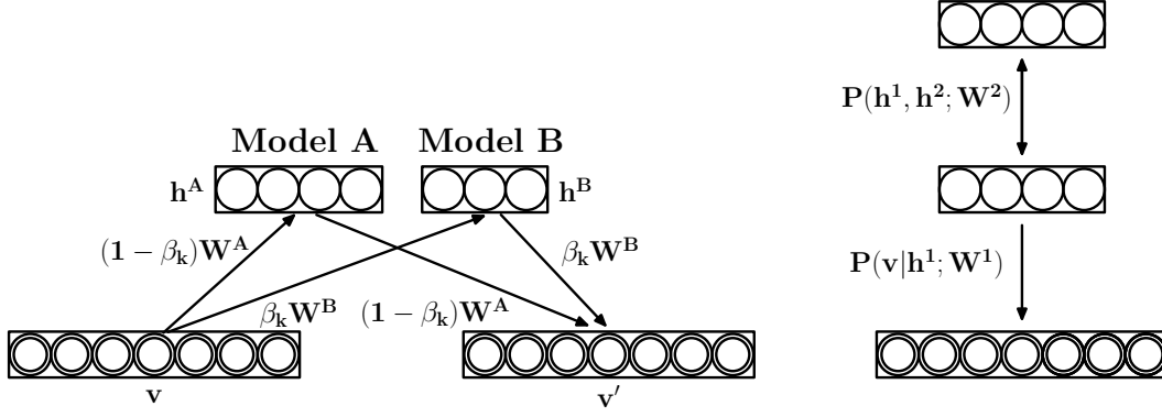
Figure 4.1: Left: The Gibbs transition operator T_k(\mathbf{v}' \leftarrow \mathbf{v}) leaves P_k(\mathbf{v}) invariant when estimating the ratio of partition functions \mathcal{Z}_B/\mathcal{Z}_A . Right: Two-hidden-layer Deep Belief Network as a generative model.
