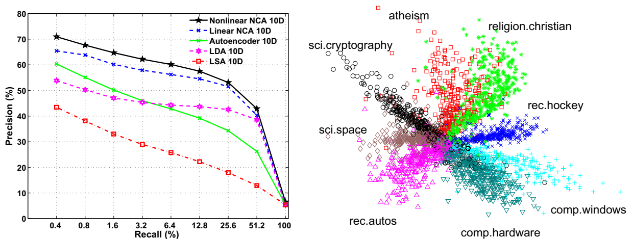
Figure 3.17: Left: Precision-Recall curves for the 20-newsgroups dataset when a query document from the test set is used to retrieve other test set documents, averaged over all 7,531 possible queries. Right: The 2-dimensional codes produced by nonlinear NCA on test dataset using 2000-500-500-2 encoder.
