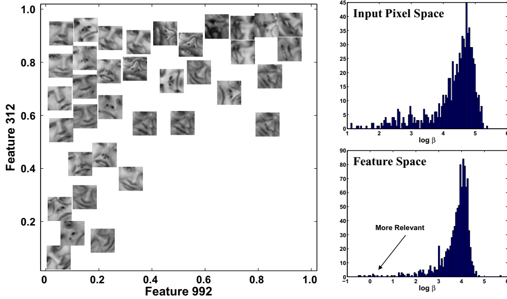
Figure 3.3: Left: A scatter plot of the two most relevant features, with each point replaced by the corresponding input test image. For better visualization, overlapped images are not shown. Right: The histogram plots of the learned ARD hyper-parameters \log \beta .
