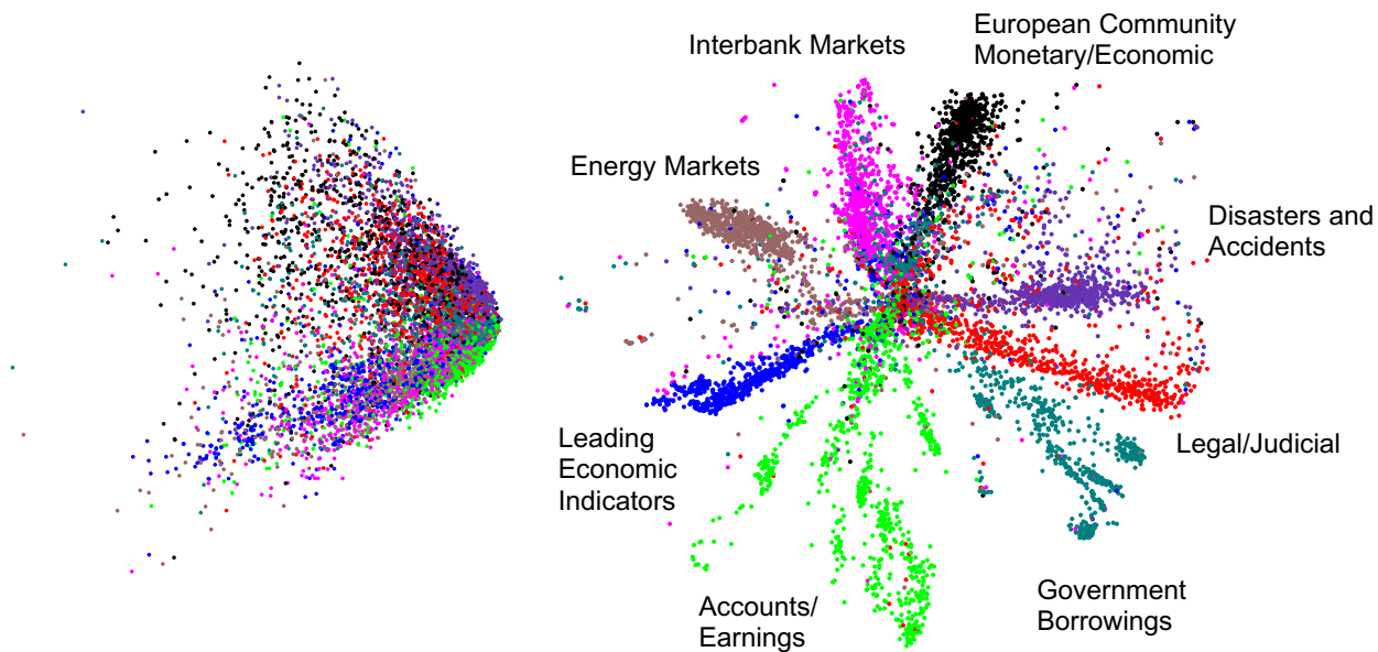
Figure 3.10: Left: The codes produced by the 2-dimensional LSA. Right: The codes produced by a 2000-500-250-125-2 autoencoder.
