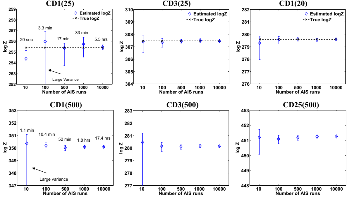
Figure 4.3: Estimates of the log-partition functions \log \hat{Z} as we increase the number of annealing runs. The error bars show \log(\hat{Z} \pm 3\hat{\sigma}) .
