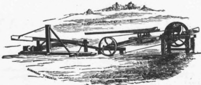
EASTWOOD & CO'S CELEBRATED TWO-HORSE POWER DRAG SAWING MACHINE, WITH STRAW CUTTER ATTACHED. Repairing done on the shortest notice. EASTWOOD & CO., Ingersoll, Ont.
